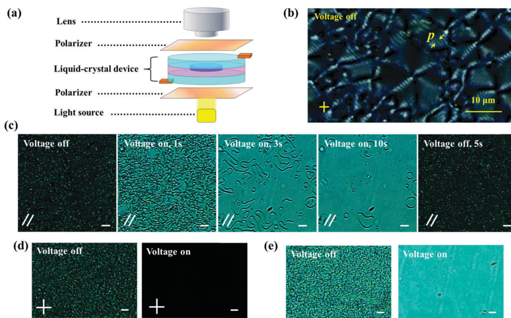
Fig. 3 Voltage-dependent microstructures. (a) Schematic of the experimental setup. (b) The focal conic texture of the cholesteric placed between perpendicular polarizers, observed at the voltage-off state. (c) Dynamic process of the cholesteric observed with parallel polarizers (Movie S2, ESI † ) at a voltage of amplitude 500 V and frequency 1 kHz. (d) Device placed between perpendicular polarizers, observed at the voltage-off and voltage-on states (Movie S3, ESI † ). (e) Device placed under the microscope without an analyzer, observed at the voltage-off and voltage-on states (Movie S4, ESI † ). Scale bars in (c)–(e) indicate 100 \mu\text{m} .
